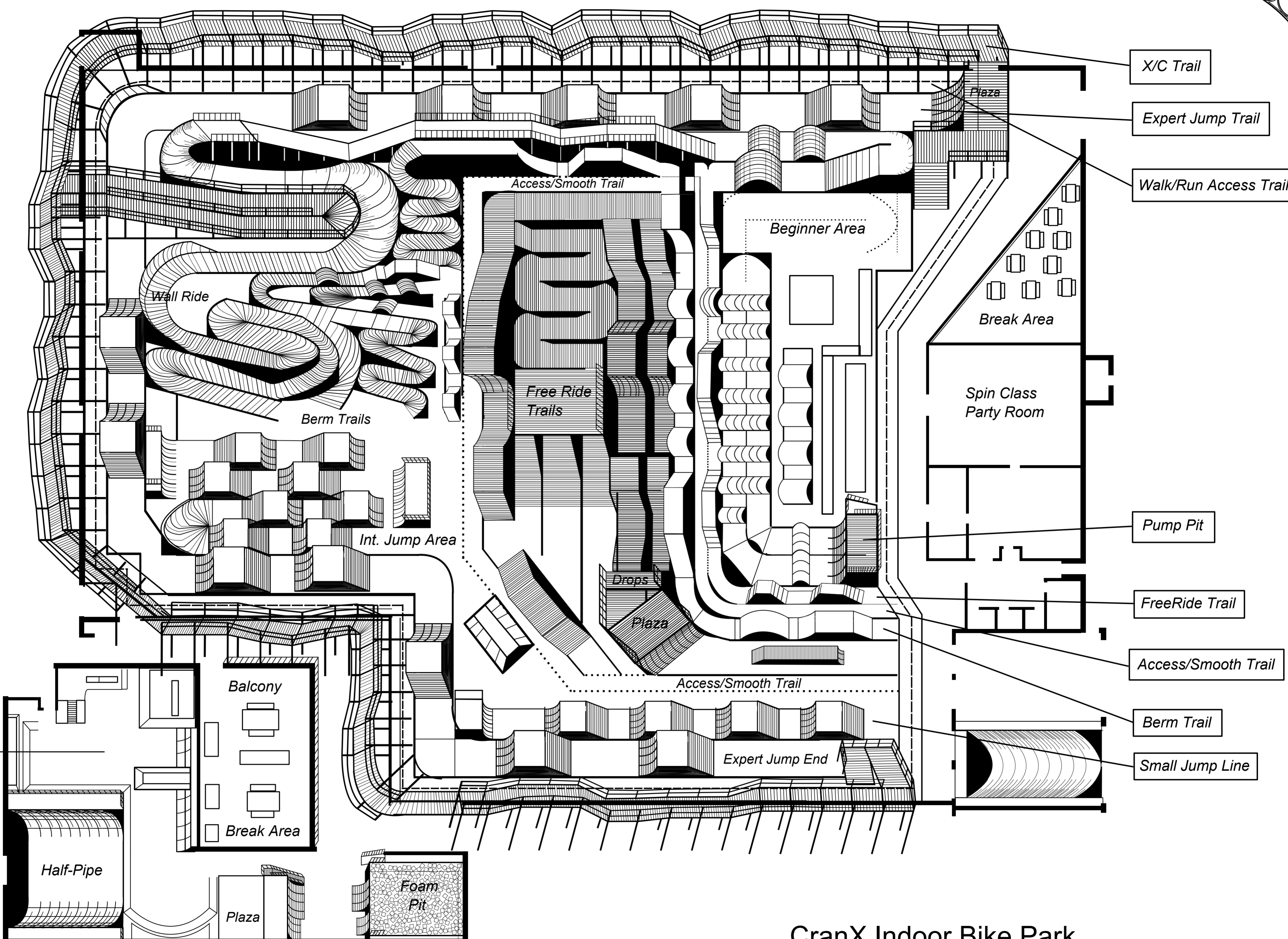
Conceptual Layout Indoor Section Phase 1
